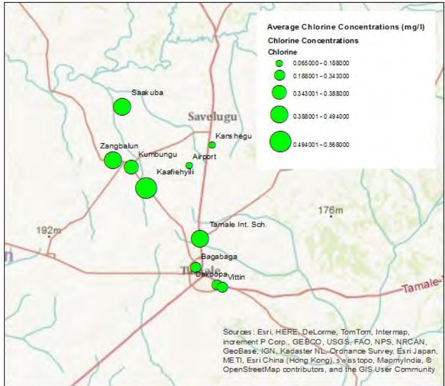
Figure 4-11: Average chlorine residual map
